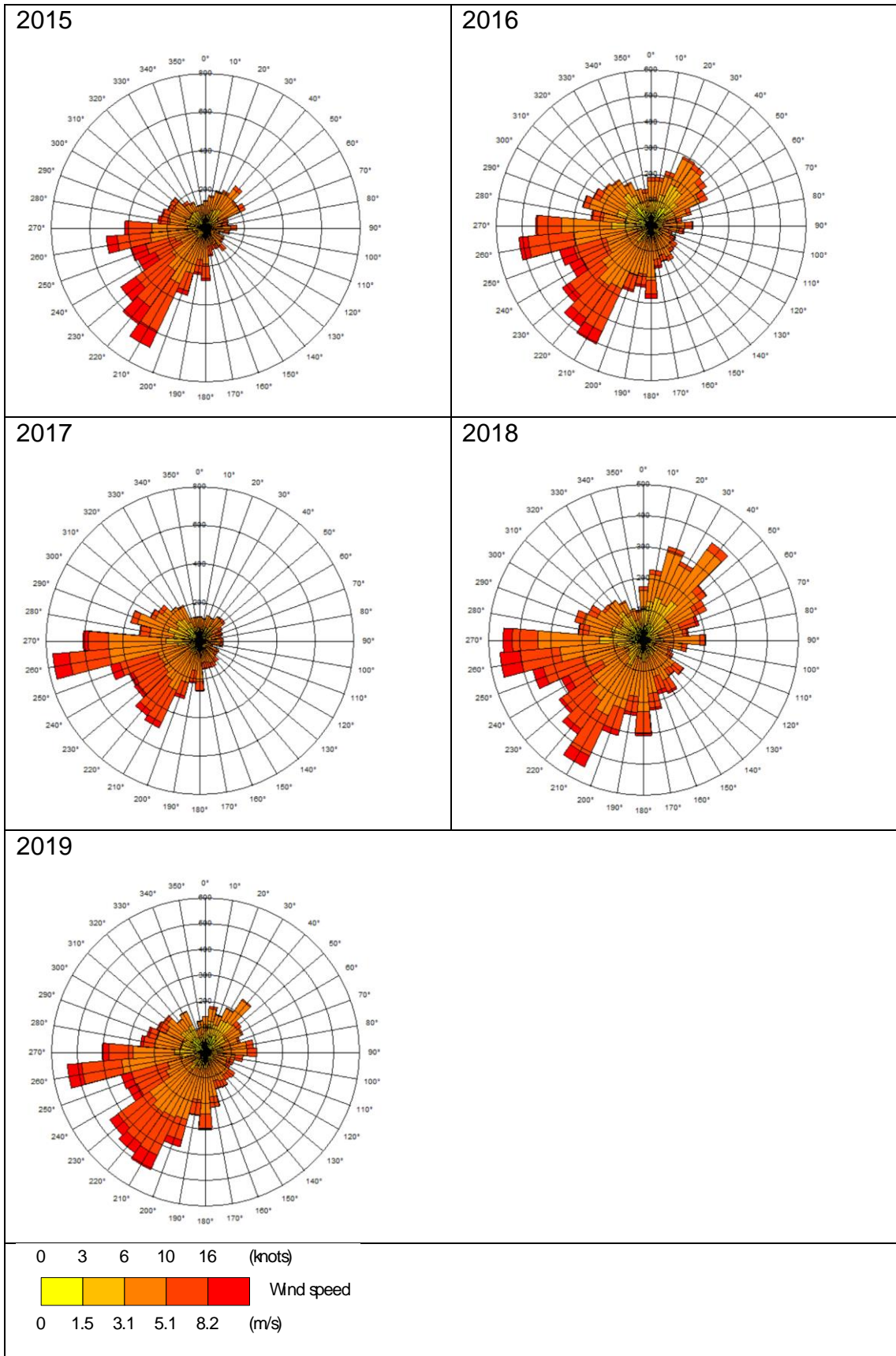
Figure 8A.1: Wind roses for Heathrow Airport, 2015 to 2019
